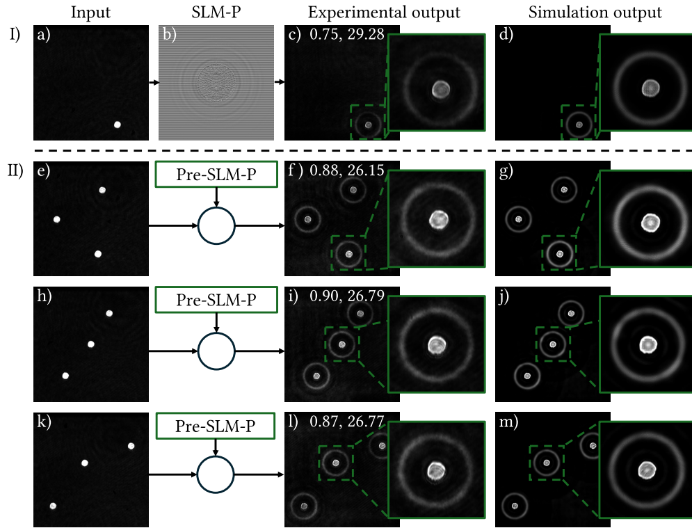
Fig. 3. Scenario 1: Object highlighting. We show the workflow of the optimization and augmentation stages. (I) Offline optimization stage, where the SLM phase is optimized to highlight the target distribution ( 30\ \mu\text{m} diameter circle). (II) Real-time augmentation stage, where the pre-computed SLM phase (Pre-SLM-P) obtained during optimization is reused on novel microscopic frames. We provide CC and PSNR values for each stage. See Visualization 1 for a live demonstration of object augmentation.
